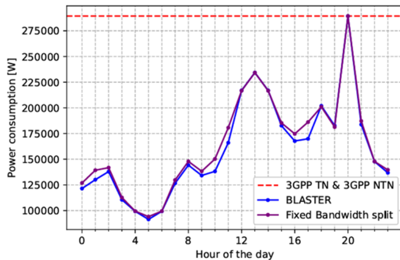
Figure 15. Network Power consumption throughout the day.
