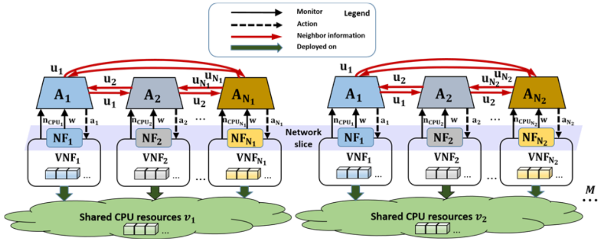
Figure 52: The Distributed Intelligence Framework for the Autoscaling System
