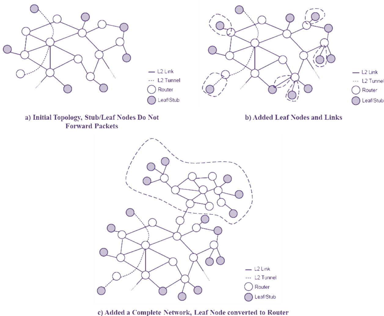
Figure 83: Large Scale Operator Network Scenario
