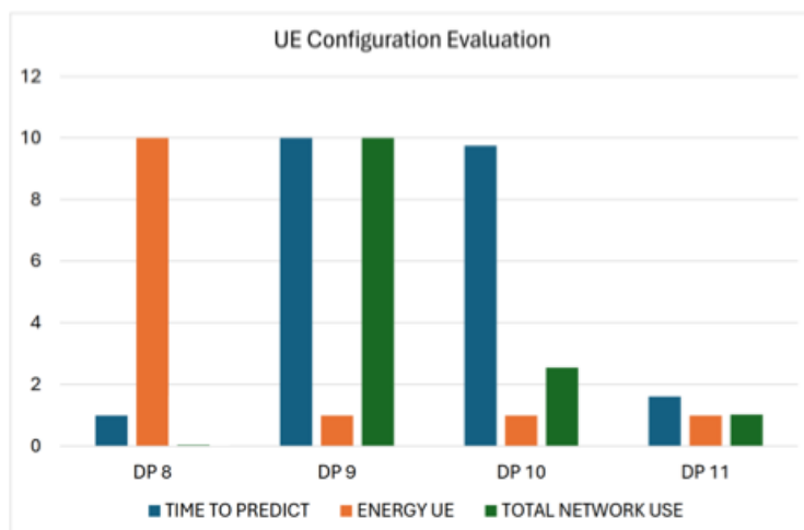
Figure 81: Placement Deployment involving UE: Comparison and Evaluation.
