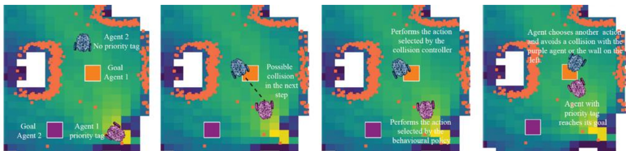
Figure 41: Explanation of the process performed by the collision controller to minimize even more the number of collisions
