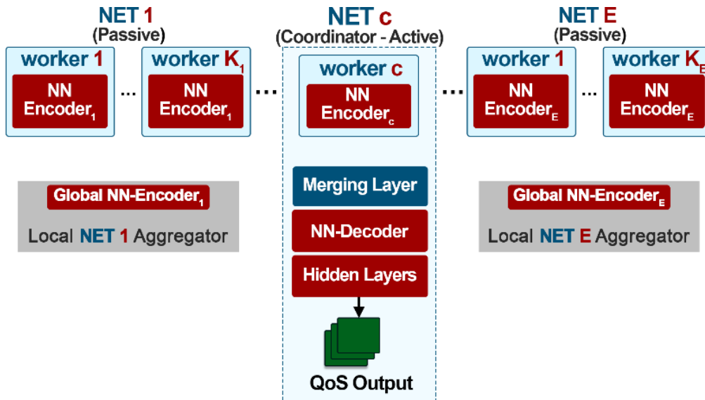
Figure 34 DISTINQT's Architecture Overview
