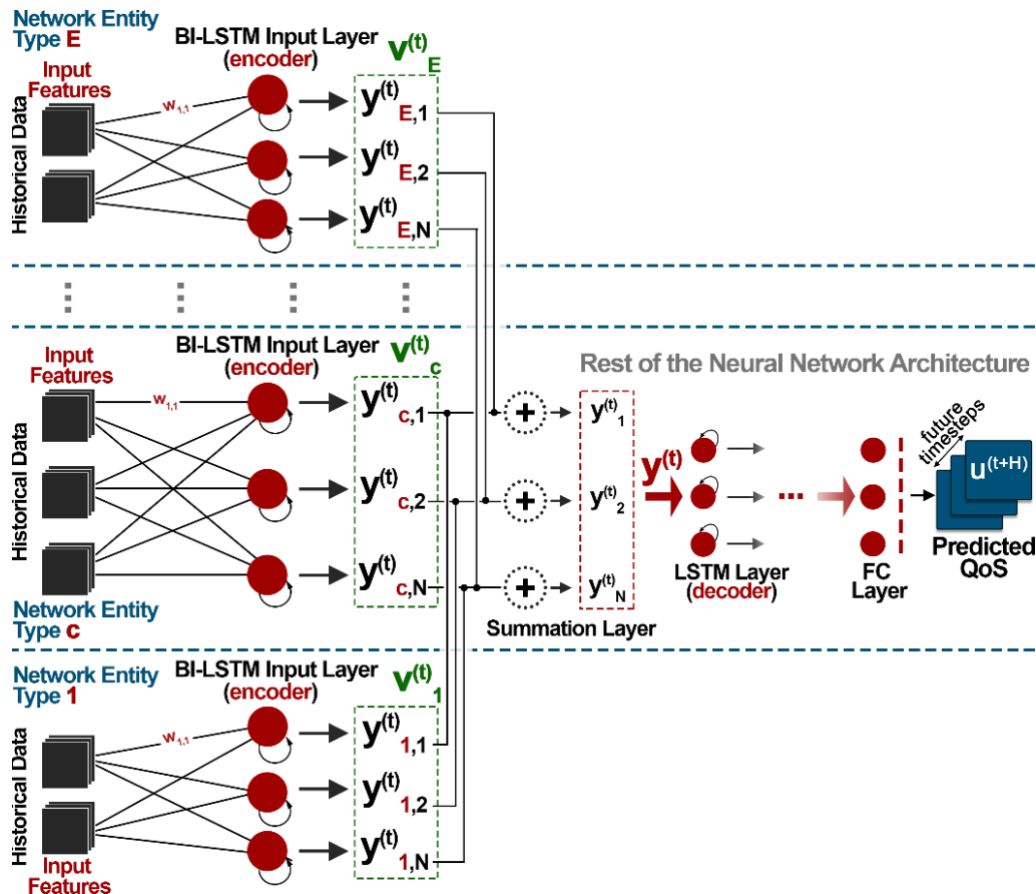
Figure 35 Distributed QoS prediction scheme
