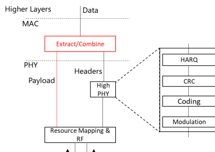
Figure 3: Data plane including Extract/Combine functions.
