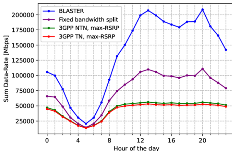
Figure 16. Network Sum Data-Rate throughout the day.
