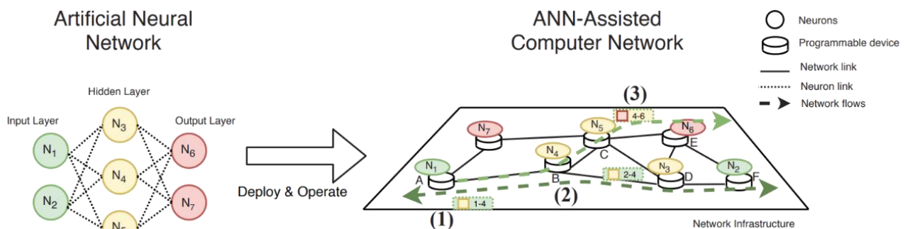
Figure 60: Distributed ANN [43]
