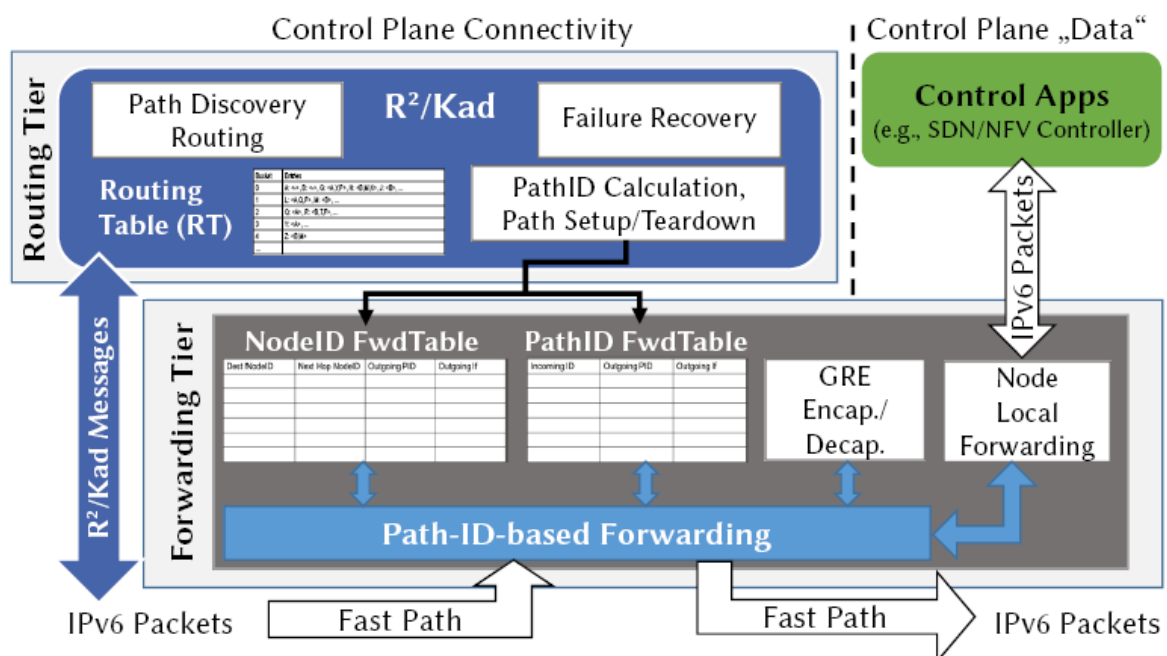
Figure 86: KIRA Architecture [30]
