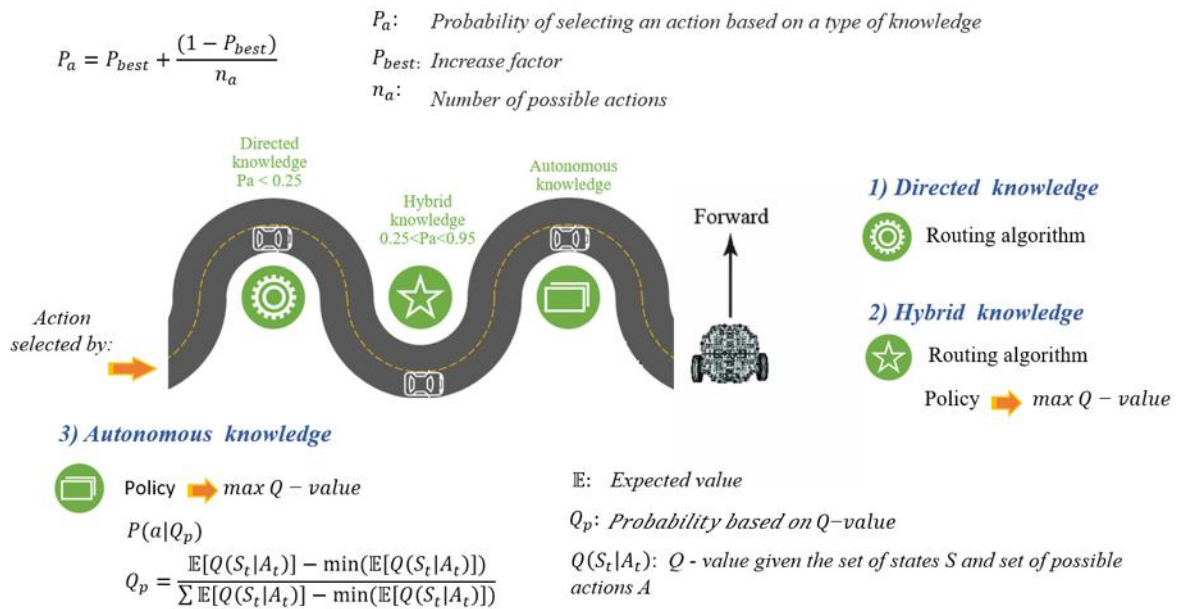
Figure 37: Description of the transition process from exploration to exploitation through three types of knowledge
