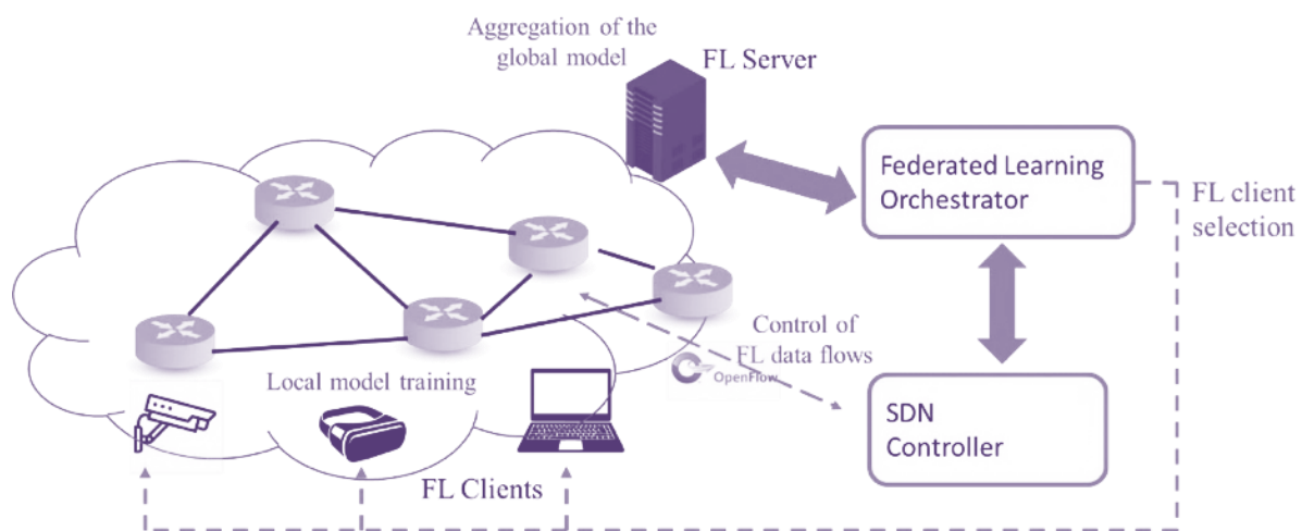
Figure 44: Possible reference scheme for research on SDN-assisted FL Client Selection.
