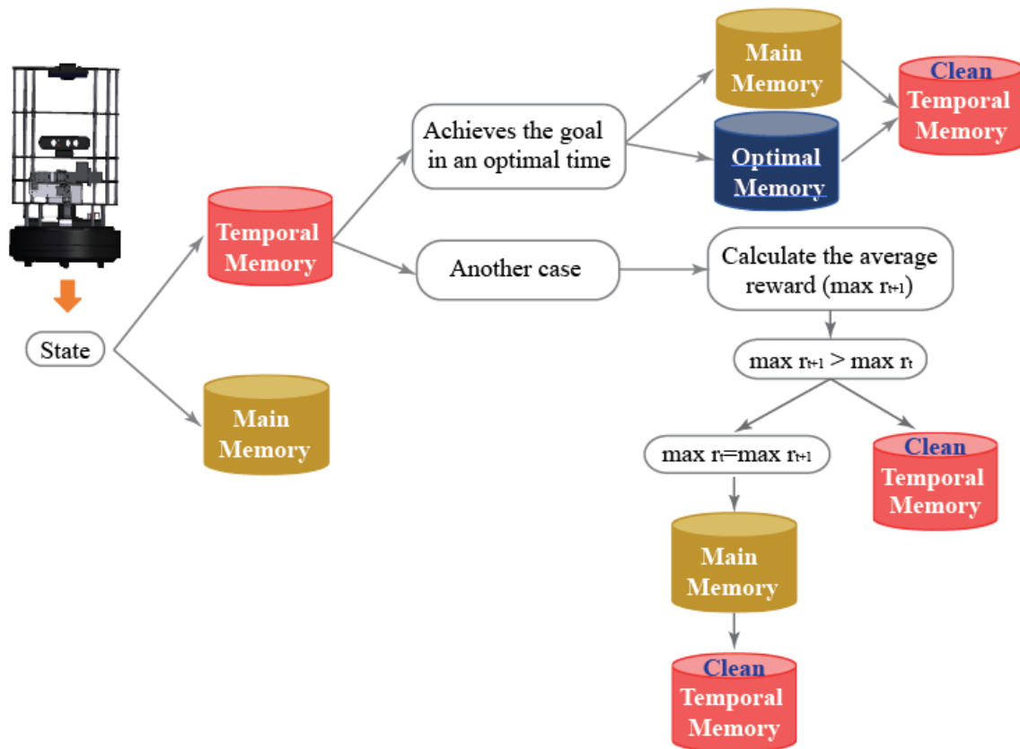
Figure 38: Description of the process of storing data collected by the agent in three different memories depending on the trajectory performed by the agent
