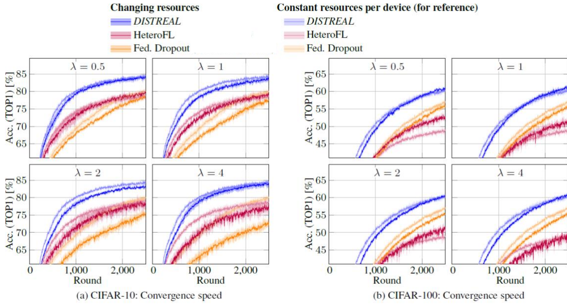
Figure 46: Convergence with CIFAR-10 and CIFAR-100 on heterogeneous devices where resources availability changes randomly over the time with rate \lambda . DISTREAL achieves a higher convergence speed than HeteroFL [77] and Fed. Dropout [78], and the highest final accuracy.
