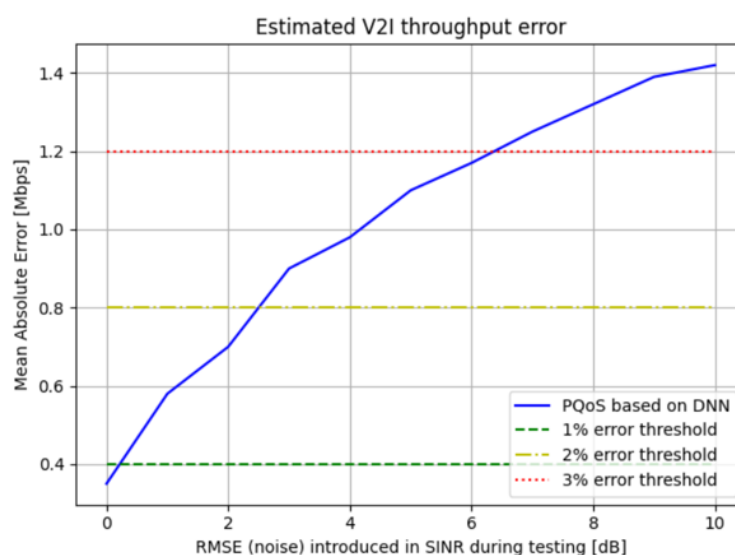
Figure 8: Benefit of Predictive QoS in estimating V2I throughput.
