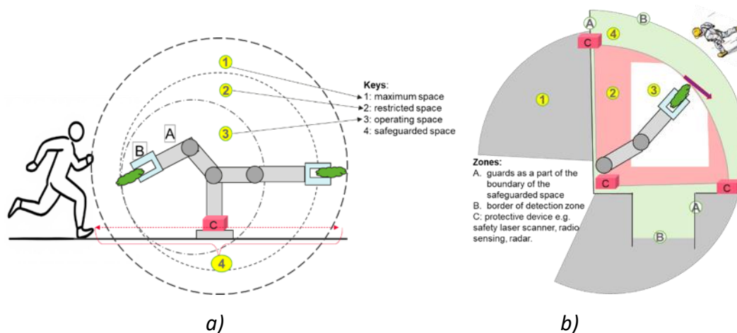
Figure 26: Dynamic Safety Zones (a- Illustrations all “spaces” associated with a robot application, b- Collaborative Applications and Permitted Zones) [ISO 10218-1]
