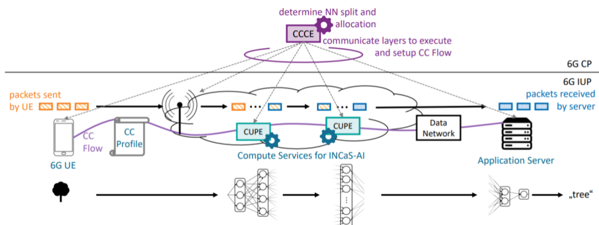
Figure 70: CC Flow for Split-AI: Execution of Neural Network parts as Compute Services [51]
