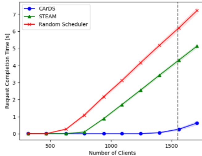
Figure 89: Runtime scheduling performance
