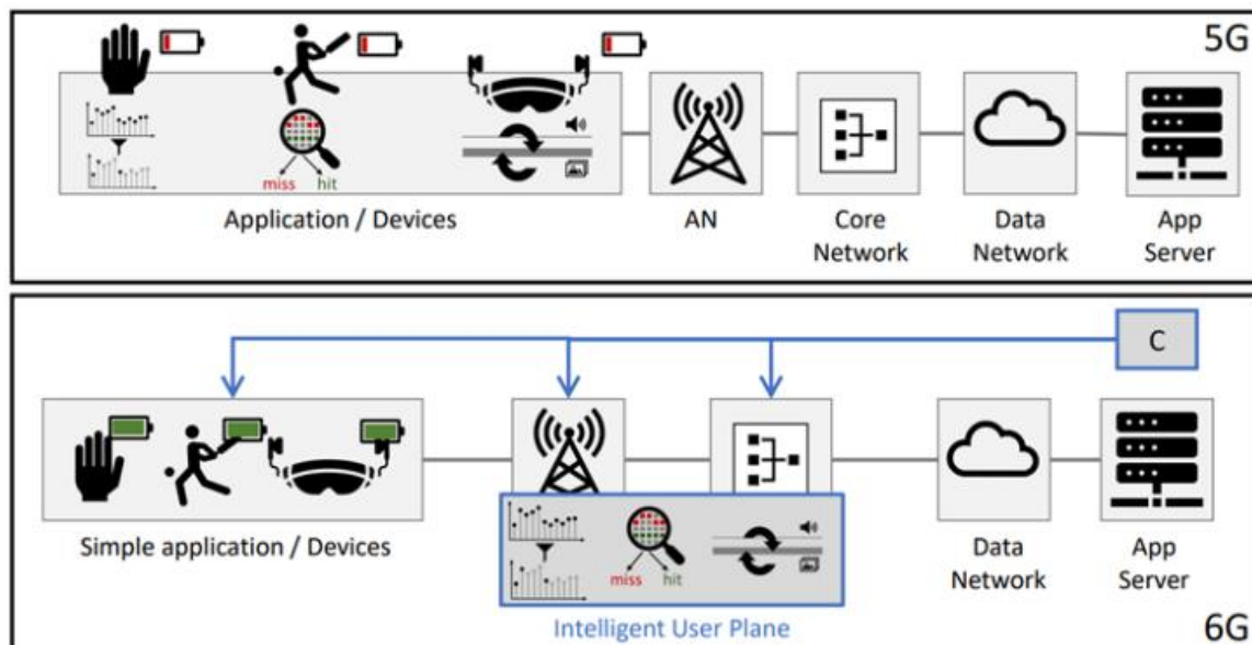
Figure 64: Intelligent User Plane to offload application-specific tasks to the UP elements
