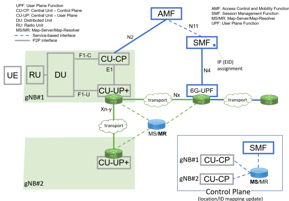
Figure 63: Proposed 6G User Plane architecture to delegate UP functionalities to the transport network
