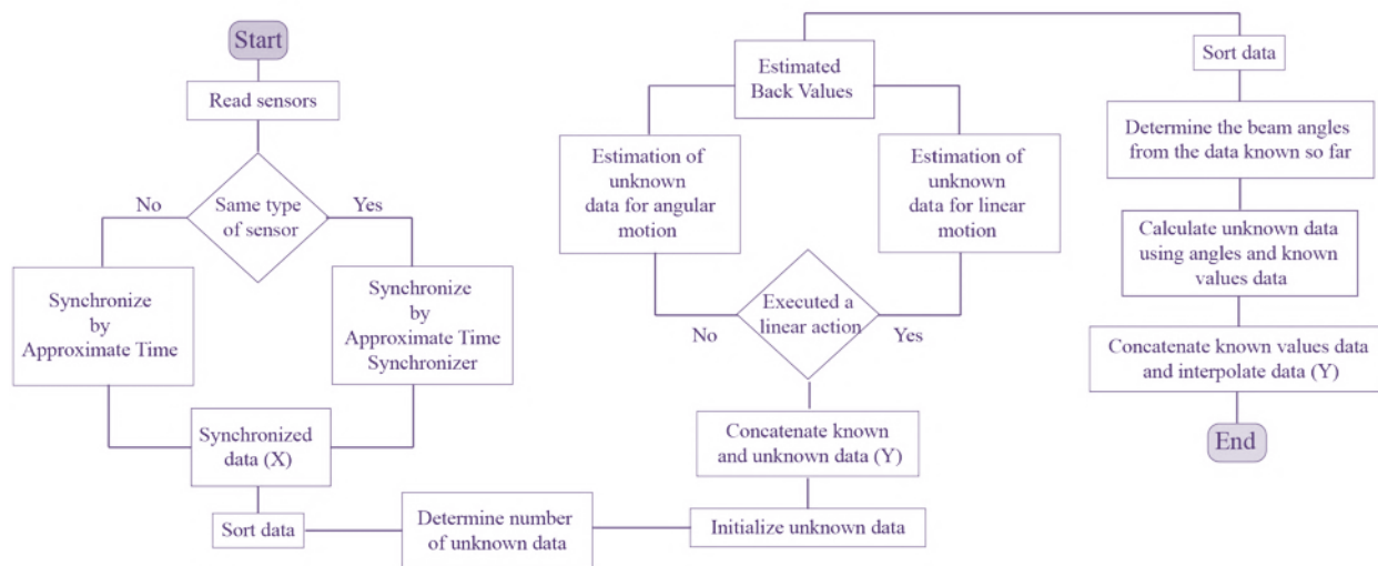
Figure 42: Process of data homogenization, synchronization and estimation proposed in [102]
