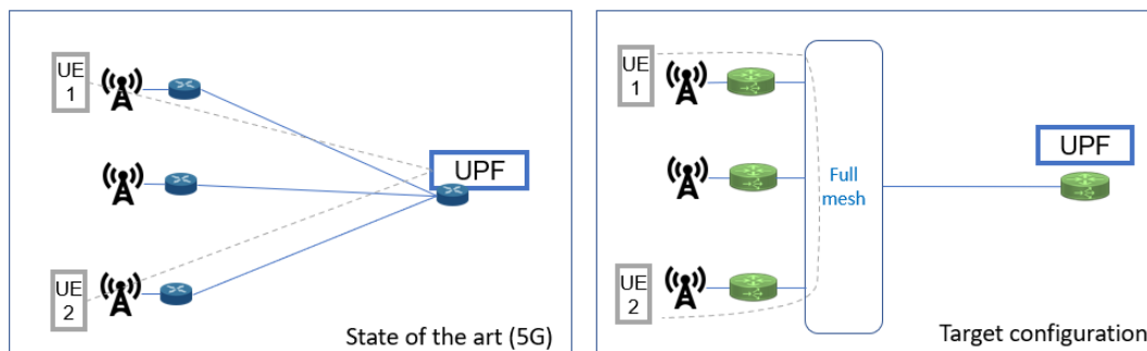
Figure 61: UE-to-UE communication in legacy and future architecture
