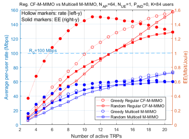
Figure 7: Rate (right y-axis) and spectral efficiency (left y-axis) of Regular CF-mMIMO vs Multicell Massive MIMO.
