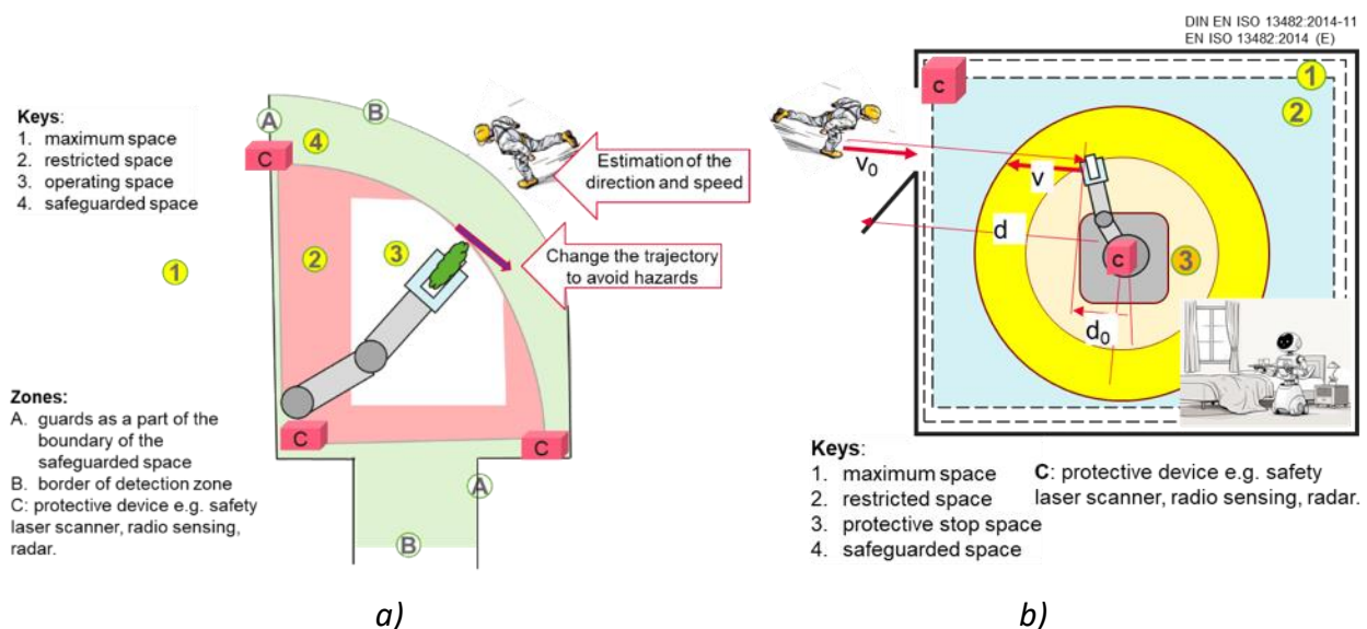
Figure 27: (a) A safeguarded space, guards and end-effector device, (b) DSZ for personal care robot. (note: 1. maximum, 2. Restricted, 3. operating, 4. Safeguard spaces)
