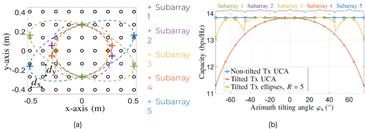
Figure 5: (a) Example of R = 5 subarrays in different colours that can compensate different tilts at a fixed Tx-Rx distance of 53.8 m. A grid of antennas can also be used to approximate different subarrays. (b) Performance enhancement by selecting different subarrays at different tilting angles
