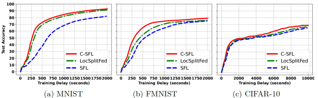
Figure 49: Test accuracy versus training delay
