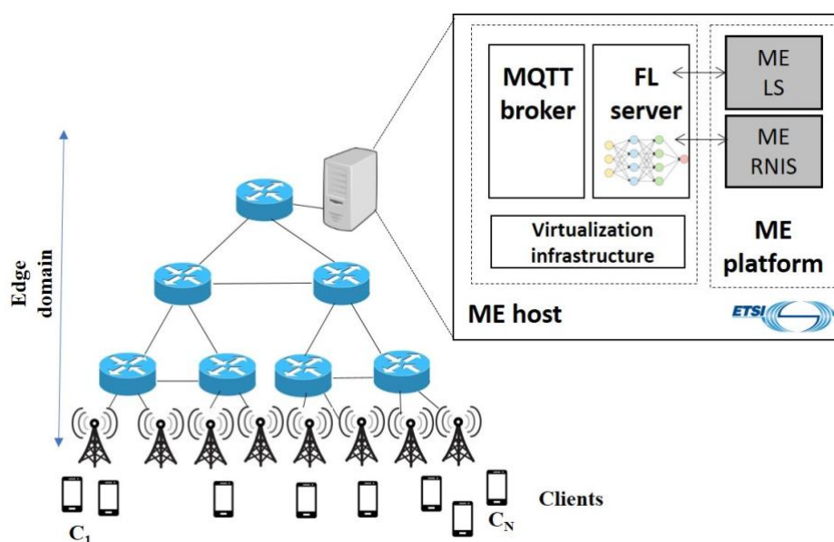
Figure 43: Reference architecture for research on Edge-assisted MQTT-based Client Discovery [73]
