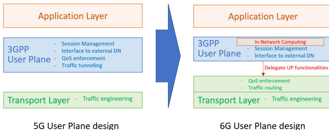
Figure 82: Potential 6G User Plane design in comparison to 5G state of the art
