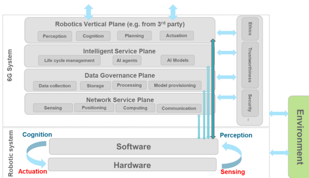
Figure 28: High Level Architecture (Revised from [5])
