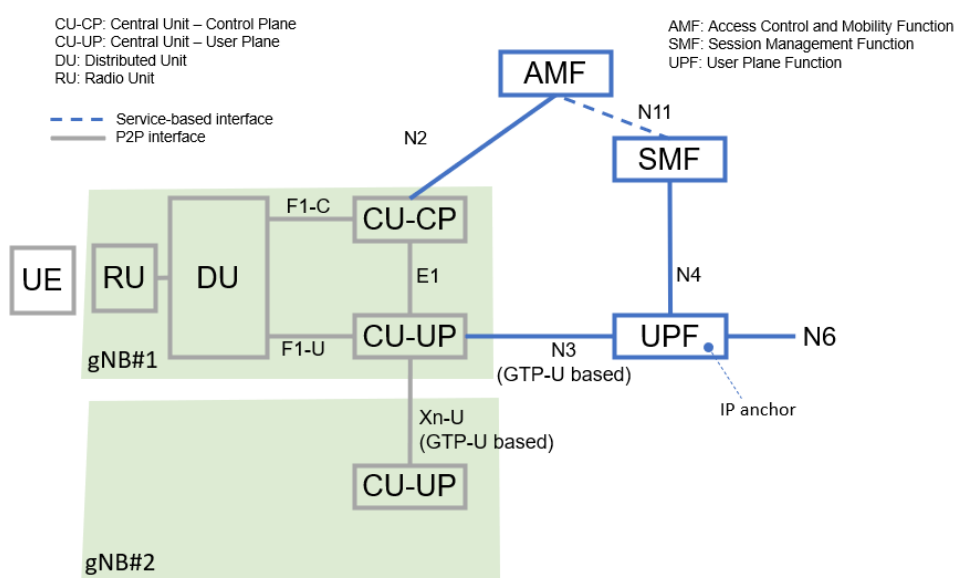
Figure 62: 5G state of the art architecture (simplified view)
