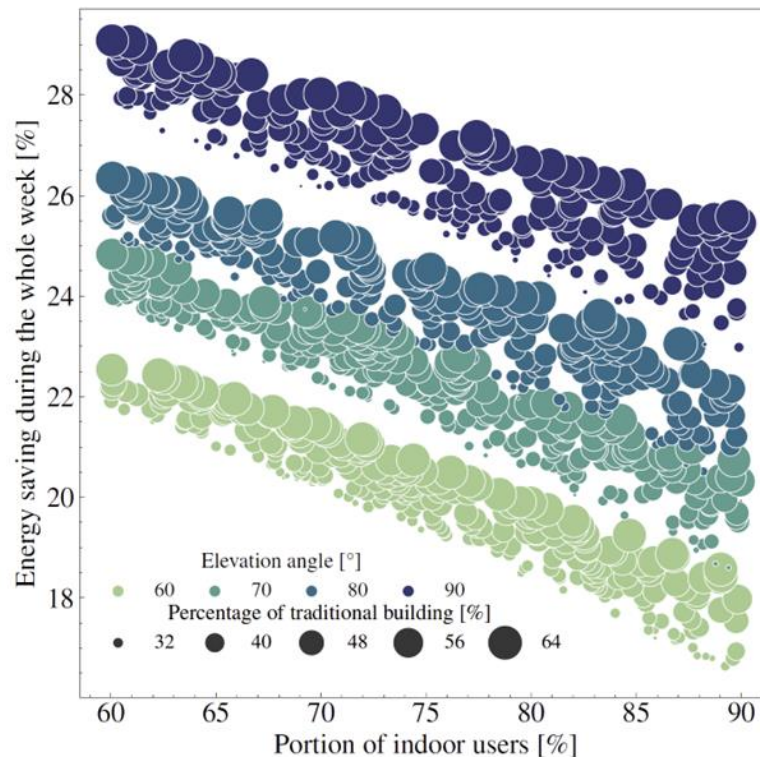
Figure 14. Energy saving at each trial (y-axis) with respect to elevation angle (sample color: the darker the color, the larger the angle), portion of indoor users (x-axis), and percentage of traditional buildings (sample size: the larger the size, the more the traditional buildings).
