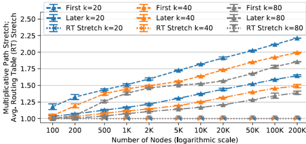
Figure 87: KIRA performance [30]
