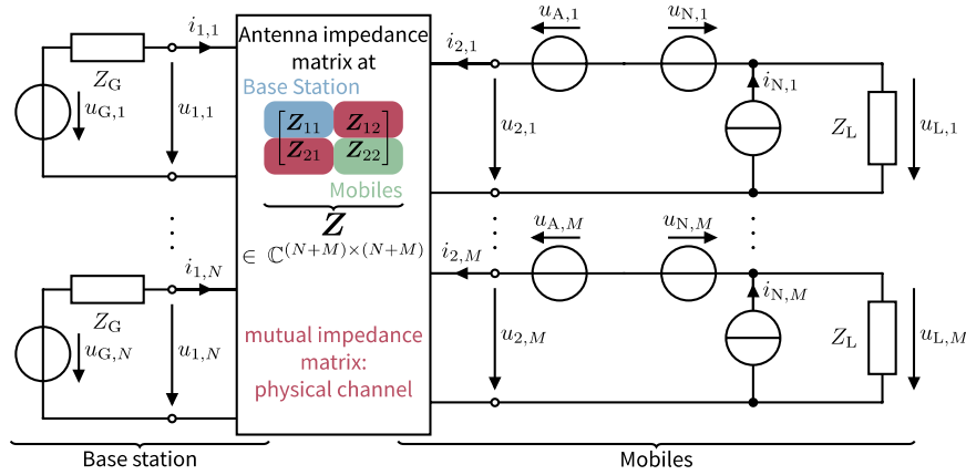
Figure 4: Circuit model in the downlink
