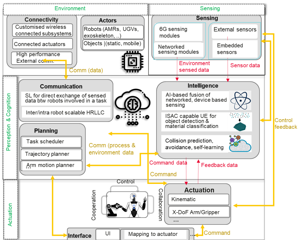
Figure 29: DSZ System Components and Functional Interactions
