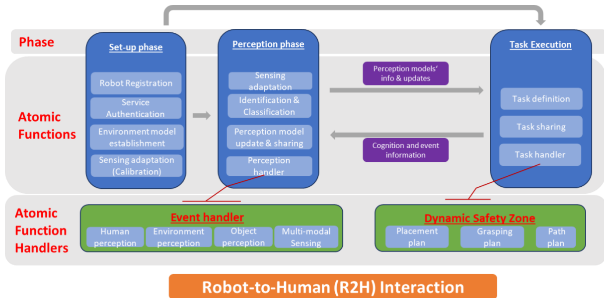
Figure 30: Atomic function & handlers for DSZs and onsite human operator
