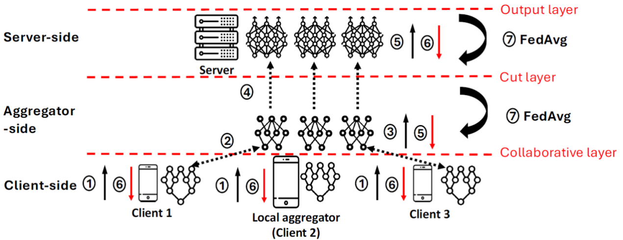
Figure 48: Clients perform forward propagation (1) and send activations to the aggregator (2). Aggregators perform forward propagation until the cut layer (3) and transmits the activations to the server (4). Backward propagation process is performed at aggregators (5), devices, and the server (6). Finally, server and aggregator models are aggregated in parallel (7).
