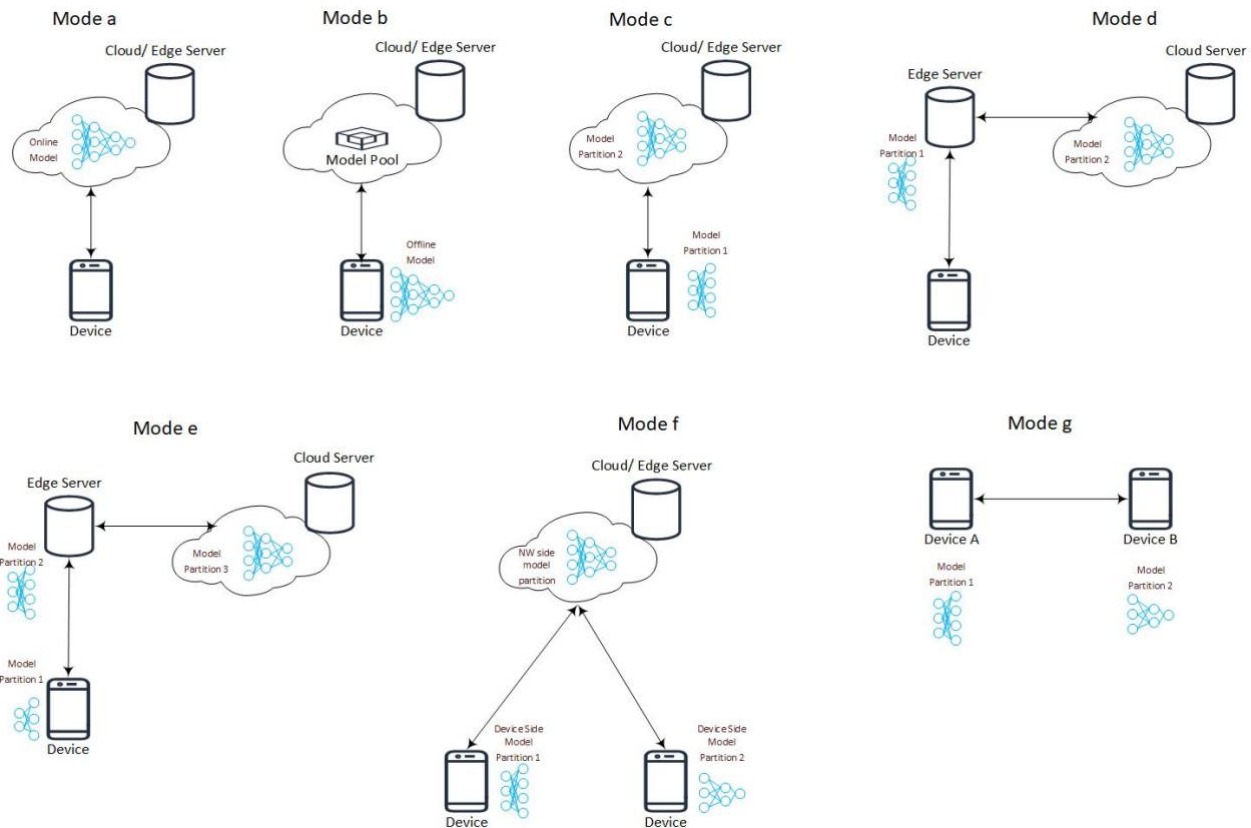
Figure 68: AI Splitting Modes [47]
