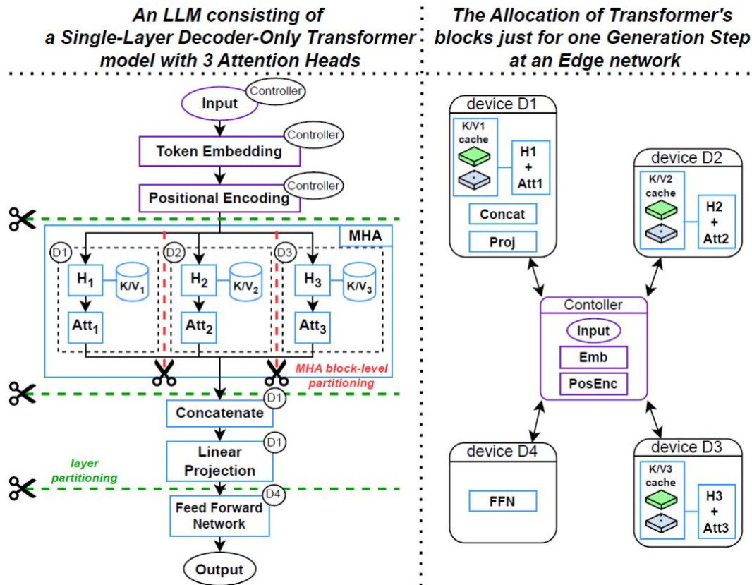
Figure 51: Illustration: attention head-level partitions (red lines) and additional cuts for feed-forward and linear projection blocks (green lines) allow flexible block assignment across edge devices. The controller node handles inference requests and partitioning, while attention heads (with K/V caches), feed forward, and projection blocks are distributed across devices D1–D4.
