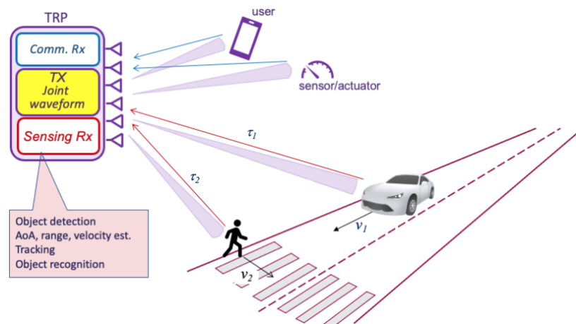
Figure 9: Joint sensing and communication in a vehicular scenario (monostatic configuration)
