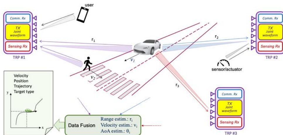
Figure 10: Joint sensing and communication in a vehicular scenario (multi-static/distributed configuration)
