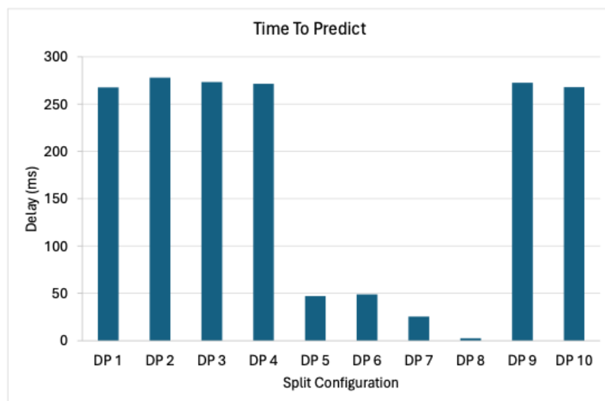
Figure 78: Time To Predict (i.e. inference delay) for each partition deployment.
